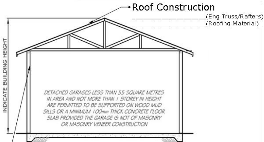
CROSS SECTION
