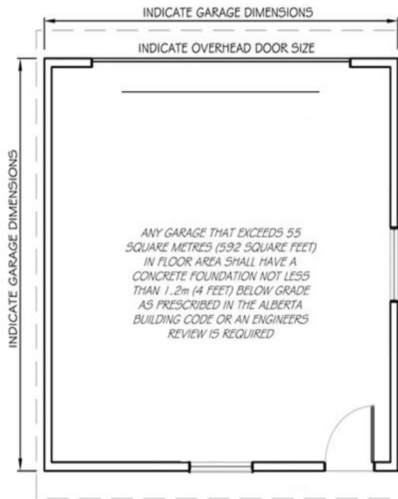
FLOOR PLAN
